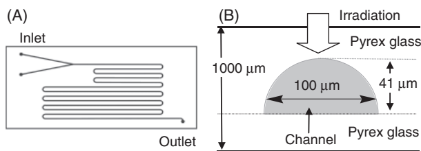
Scheme 4. (A) Top view and (B) cross section of MCR: width = 100 \mu\text{m} ; depth = 41 \mu\text{m} , length = 500 mm, volume ( V ) = 1.57 \mu\text{L} .
