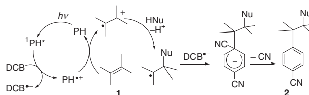
Scheme 1. Photosensitized nucleophilic addition reaction.
