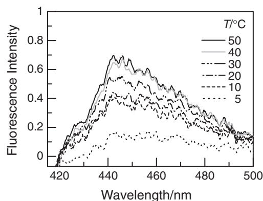
Figure 2. Temperature dependence of the exciplex emission between PH and DCB.
