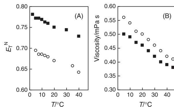
Figure 3. Temperature-dependence of (A) solvent parameter ( E_T^N ) and (B) viscosity ( \eta ) of MeCN–H 2 O (19:1) (○) and MeCN–MeOH (3:1) (■).
