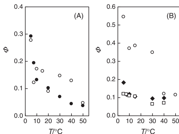
Figure 1. The temperature dependence of \Phi for (A) the formation of 2a (●) and 2b (○) from the PNA reaction of 1a and (B) the formation of 2c (○), 2d (◆), and 2e (□) from the PNA reaction of 1b .
