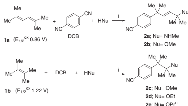
Scheme 2. The PH/DCB redox-photosensitized nucleophilic addition (PNA) of 1 in MCR: (i) hν , PH.
